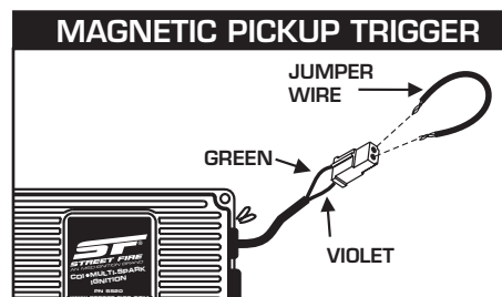
Figure 8 Checking for Spark with Magnetic Pickup.
